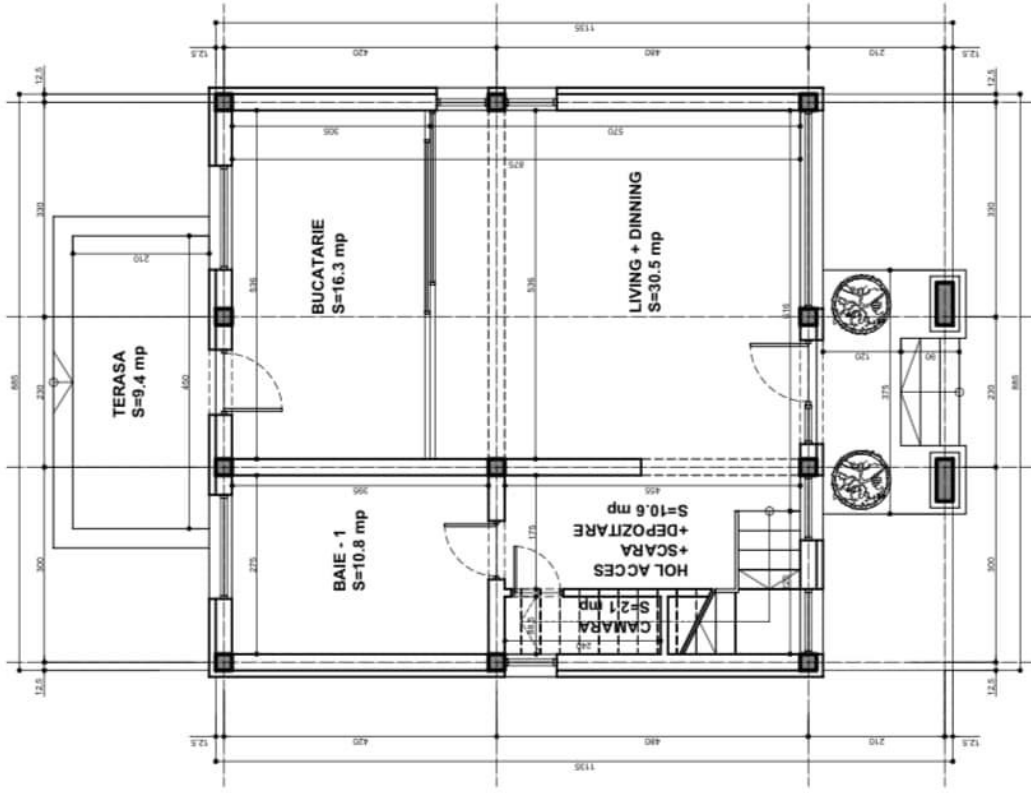
Plan parter Scara 1:50
